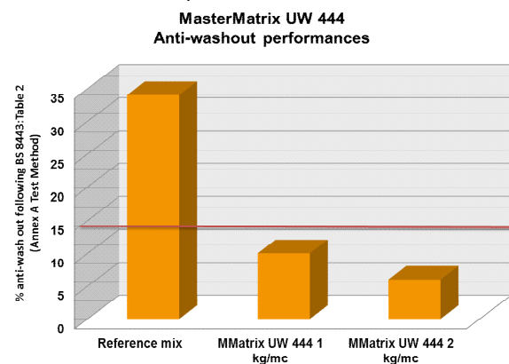
Anti Wash Out Performance of MMatrix UW 444 Dosage of cement: 400 kg/m 3 – W/C 0,52
