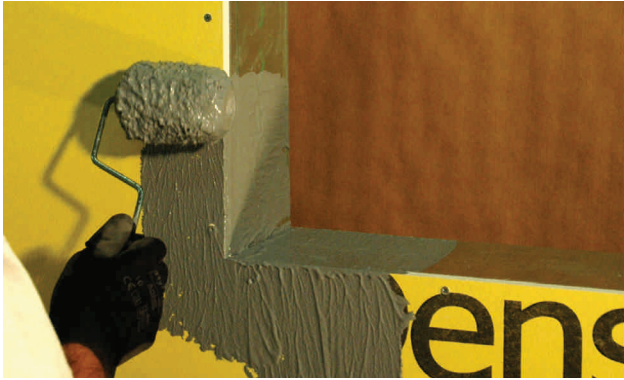
Step 1 Liberal apply fluid-applied Master Builders Solutions air/water-resistive barrier material.
