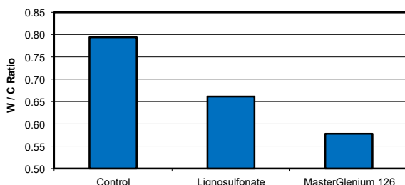
W/C Ratio Comparisons @ 1% Dosage @ S4 (180 slump)
