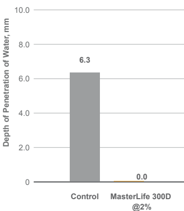
Water Penetration – DIN 1048 Part 5 (mm)
