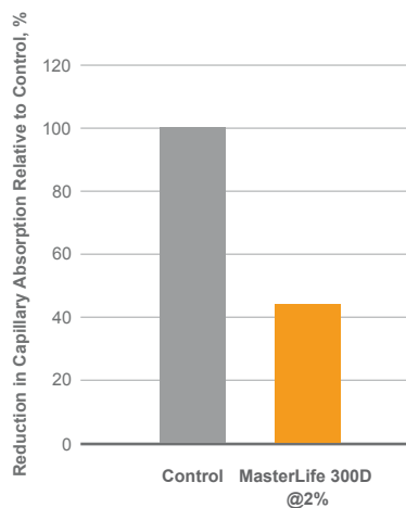
Capillary Absorption – ASTM C 1585 (%)
