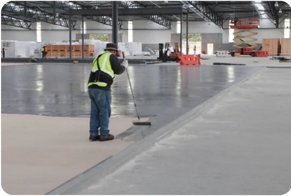
Application of Ucrete DP in the beer processing area and packaging room
